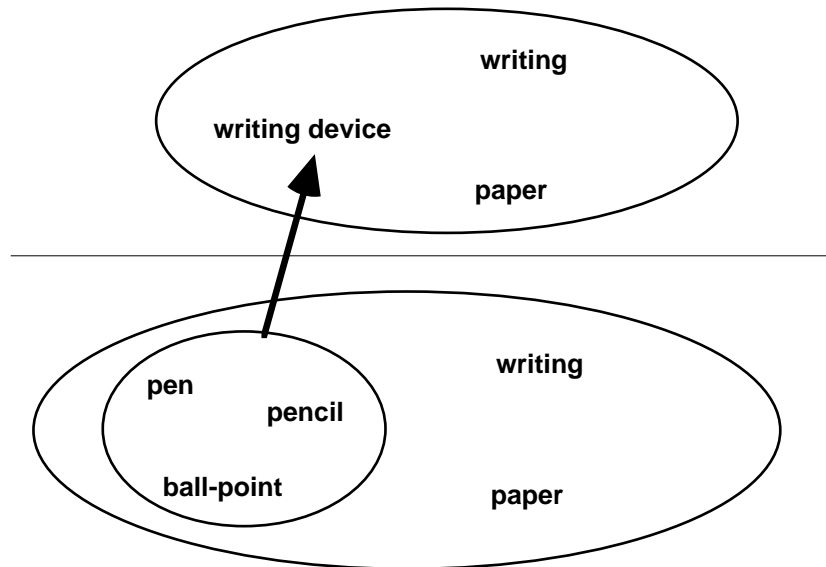
Fig. 3: a condensation of the subcoherence <pen, pencil, ball-point> into the new, more general topic writing device .
