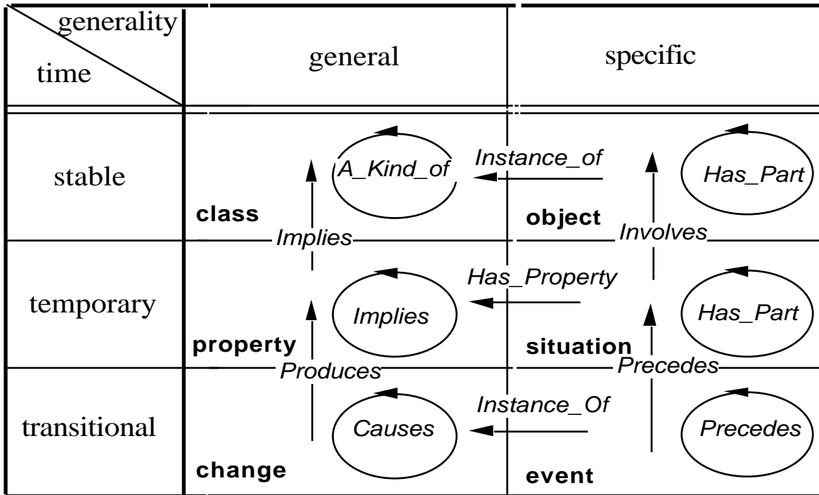
Fig. 5: Link types derived from the allowed combinations between node types; the straight arrows represent entailment from one type to another (more invariant) one, the circular arrows represent entailment from a concept of one type to a concept of the same type
