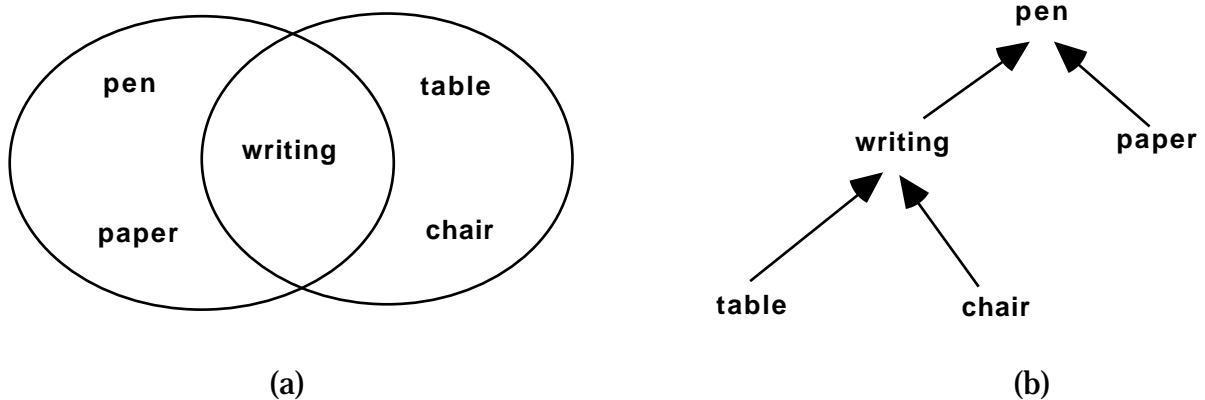
Fig. 1: (a) a simple entailment mesh consisting of two coherences overlapping on the topic writing ; (b) a 'prune' unfoldment of the same mesh from the point of view of the topic pen .
